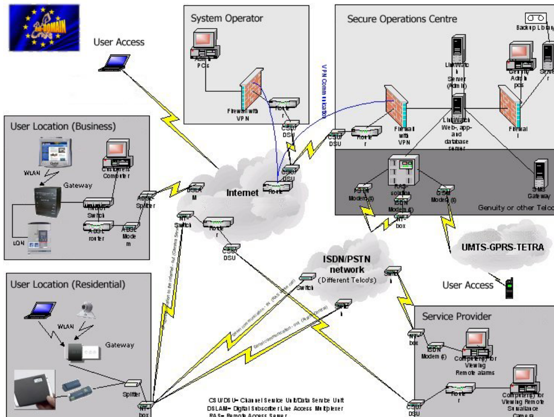
Figure 7.9: Communication infrastructure
