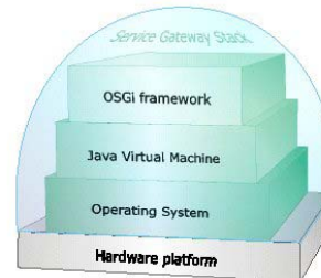
Figure 7.7: OSGi Framework
