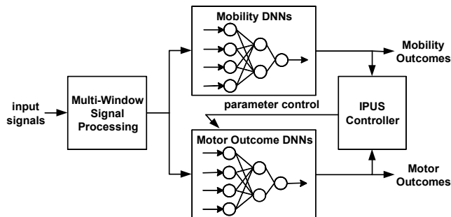
Fig. 1. Block diagram of the technology framework of the proposed system. Features are calculated across multiple time and frequency windows of the ACC and sEMG signals. These features are then fed into DNNs trained to detect the patient's mobility and motor states. The parameters controlling these DNNs are set by a rule-based IPUS controller, and adjusted according to the system outputs.
