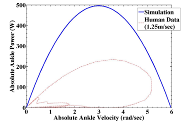
(b) Absolute Joint Power vs. Absolute Joint Velocity
