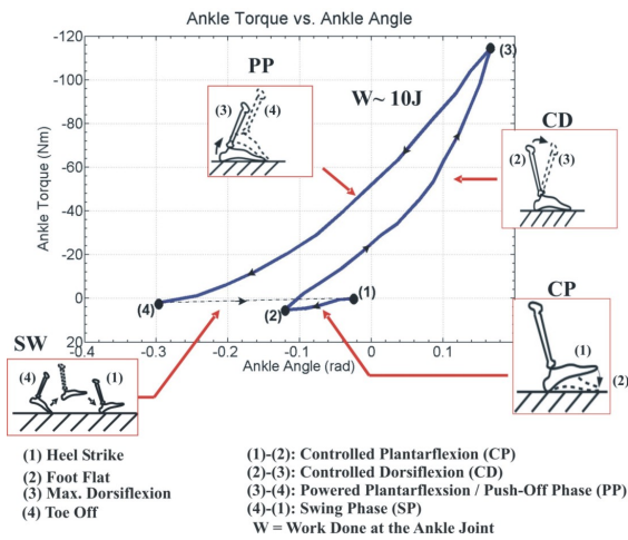
Fig. 1. A typical ankle torque-angle behaviour for a 75 kg person at his/her self-selected walking speed (1.25 m/s). Data are from [3], re-plotted in the manner of [14]. The solid line shows the ankle torque-angle behaviour during stance while the dash line shows the ankle behaviour during the swing phase.
