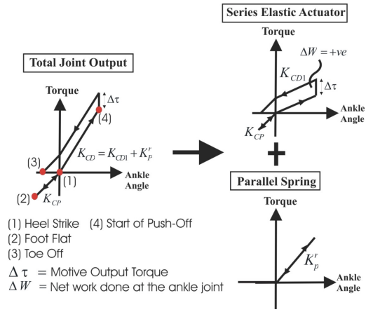
Fig. 4. Exploiting the parallel and series elasticity with an actuator.
