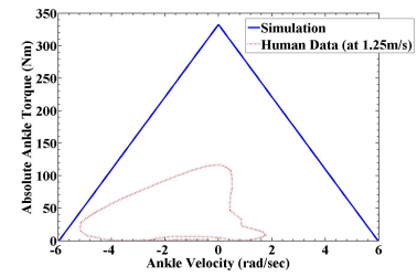
(a) Absolute Joint Torque vs. Joint Velocity
