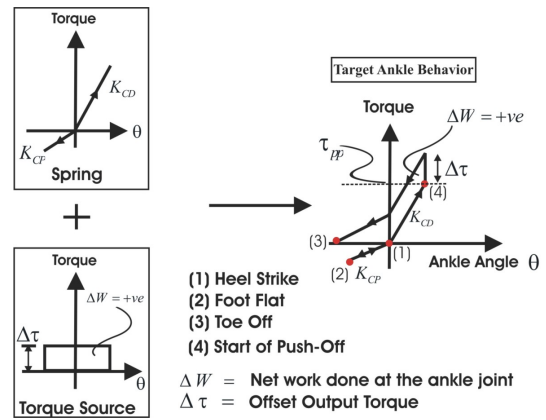
Fig. 2. Target stance phase behavior.
